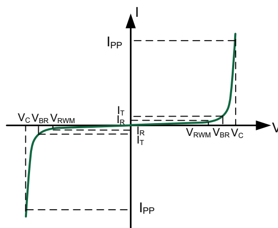
Bi-Directional TVS
