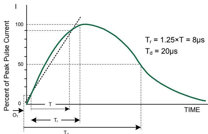
8/20μs Waveform per IEC61000-4-5
